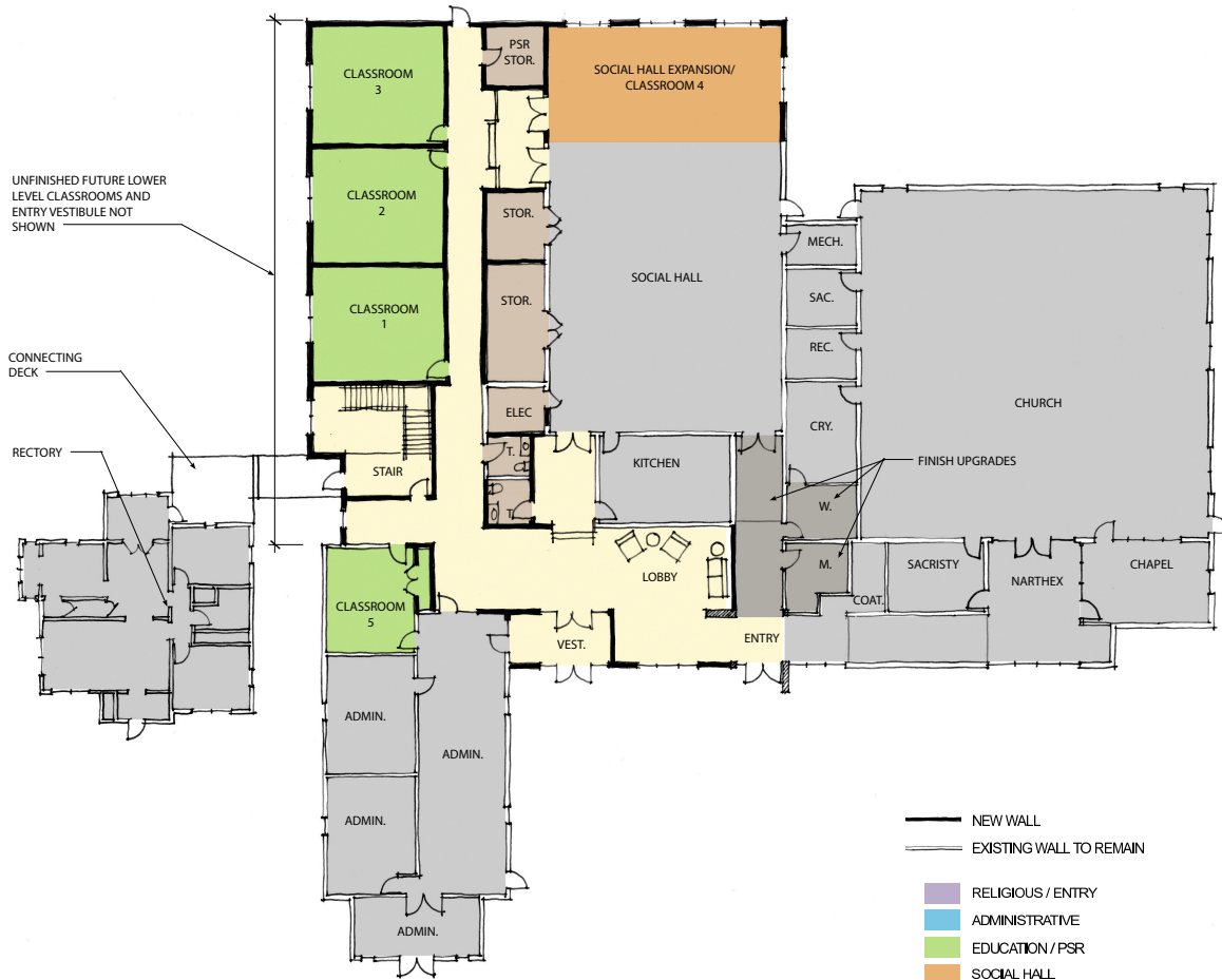
FIRST FLOOR PLAN - PHASE 1
